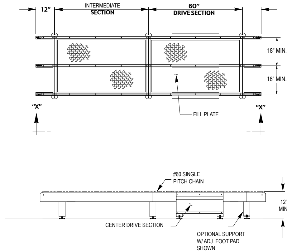
SECTION X-X
