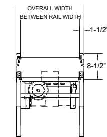
SECTION "X-X"
